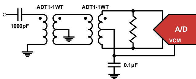
FIGURE 28. TRANSFORMER INPUT FOR GENERAL PURPOSE APPLICATIONS
