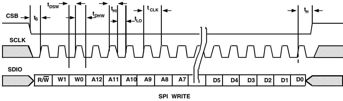
FIGURE 38. SPI WRITE
